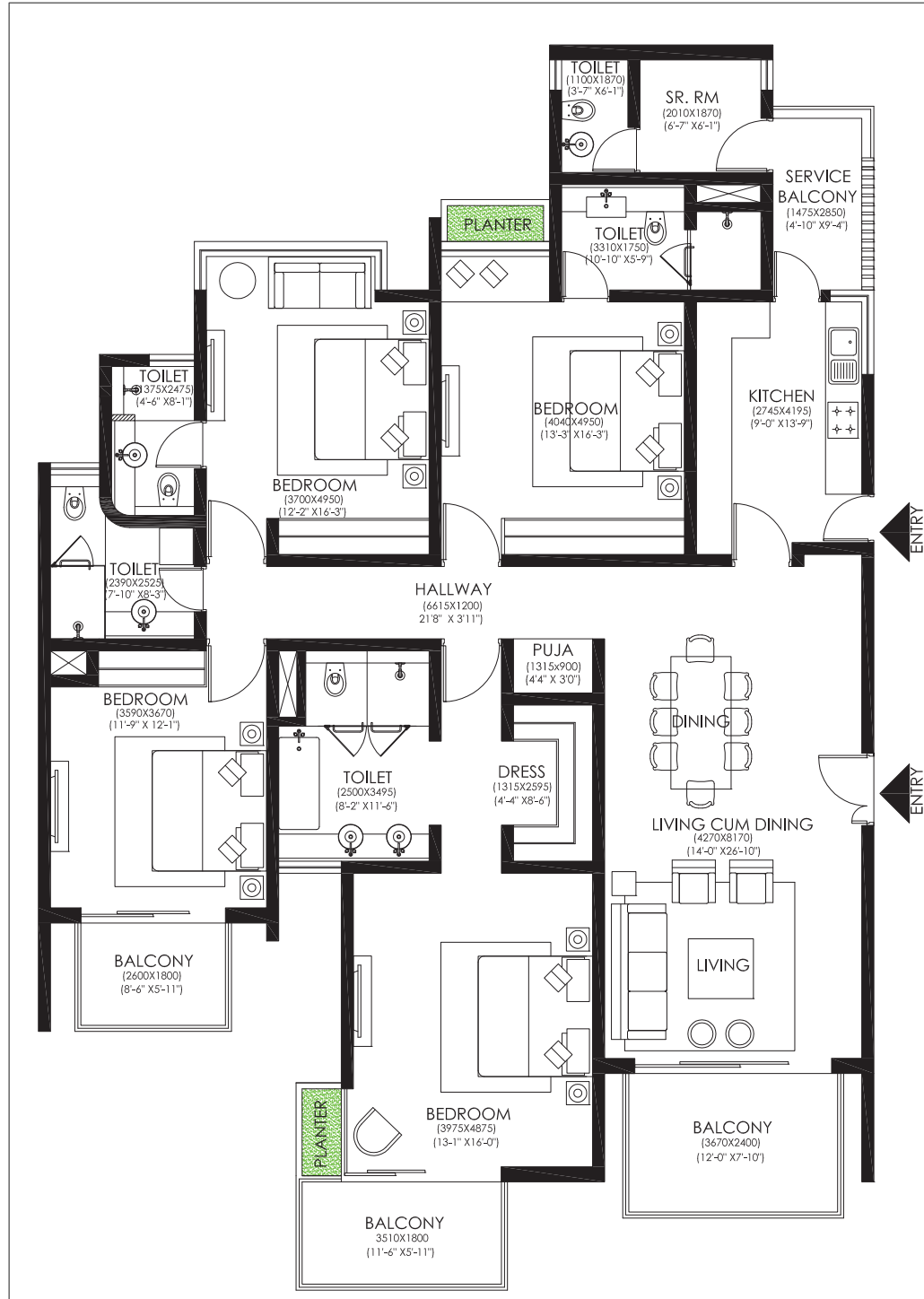
TYPICAL FLOOR PLAN OF 4BHK UNIT MID-RISE
